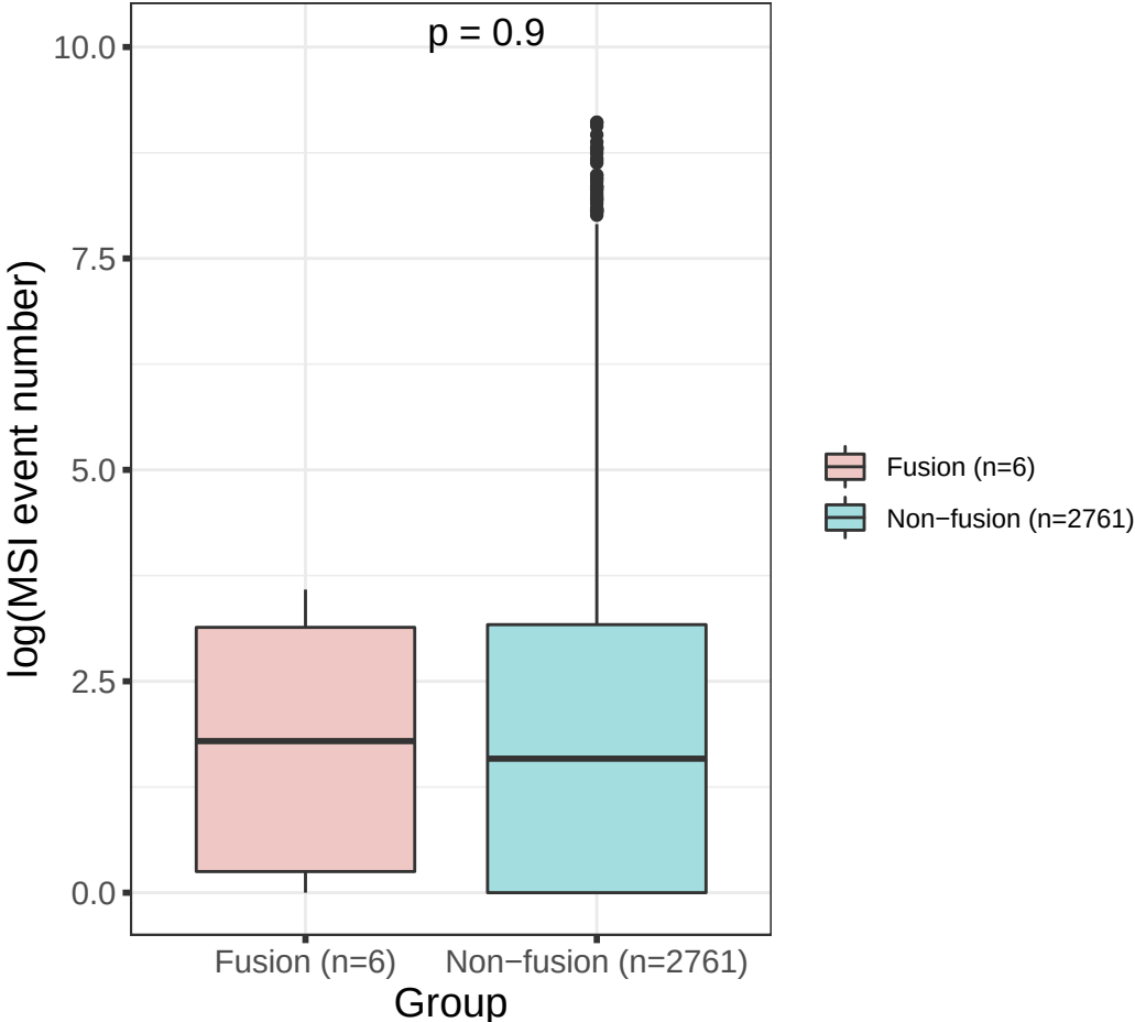
Microsatellite instability(MSI) comparison between fusion and nonfusion group
