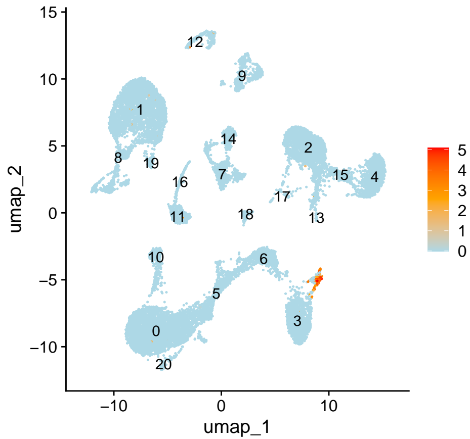
S100A9
