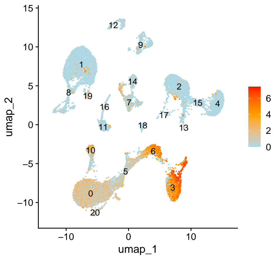
S100A9
