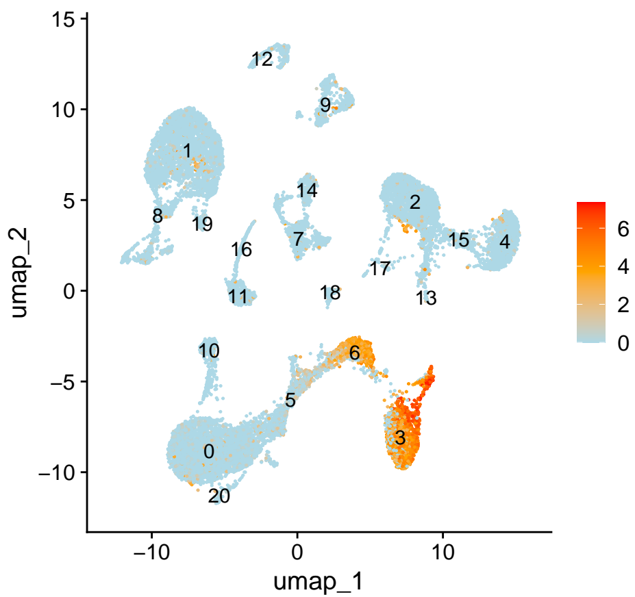
S100A8
