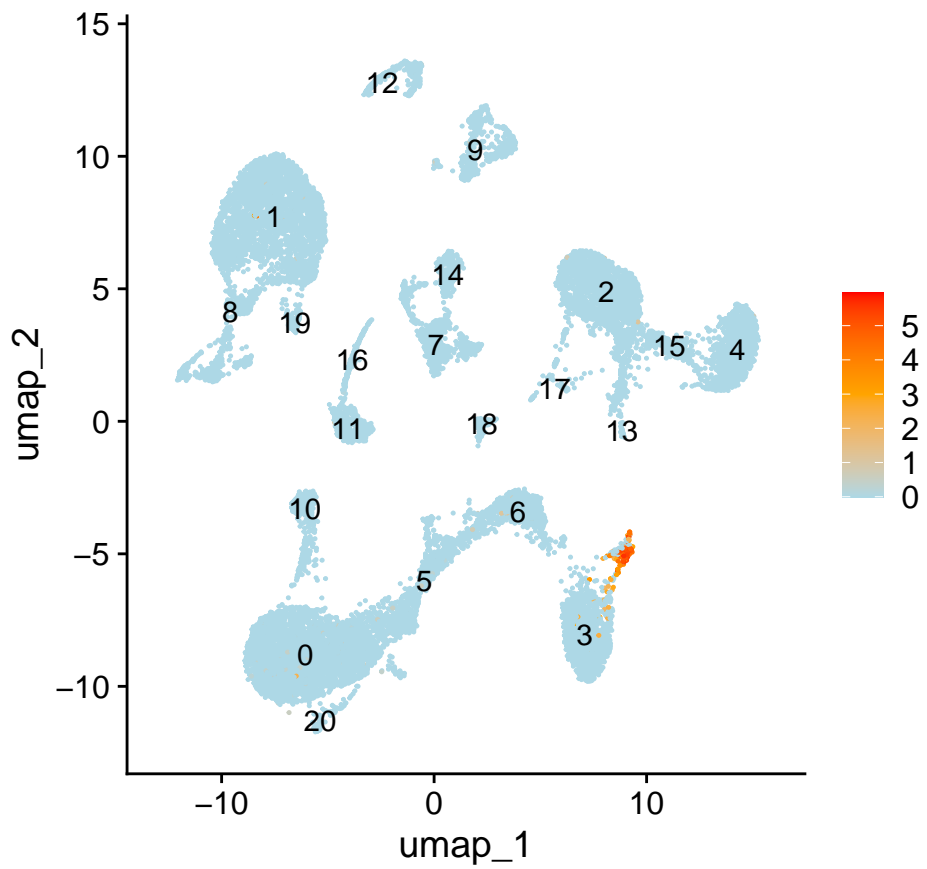
S100A8
