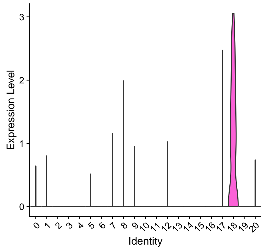
COL19A1
