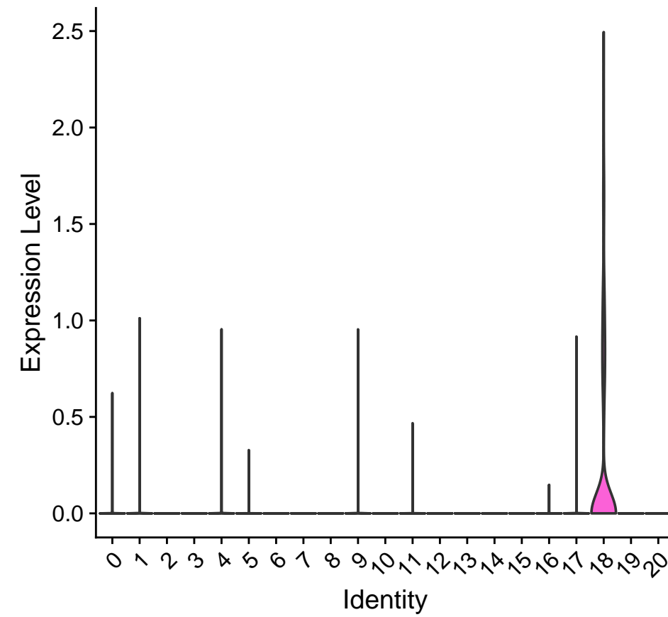
FCRL2
