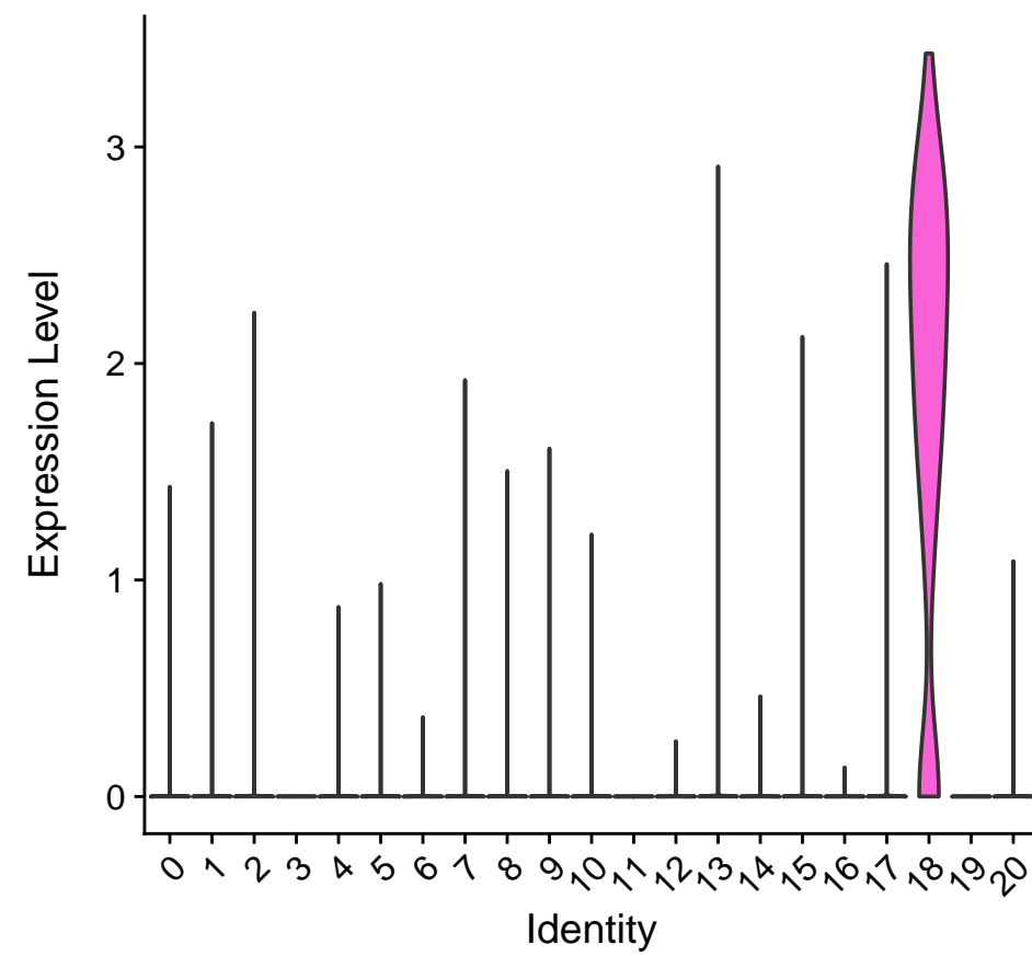
PAX5
