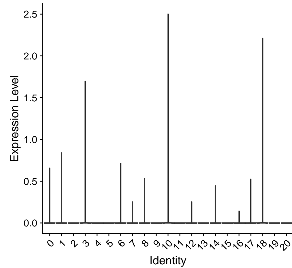
LINC01781
