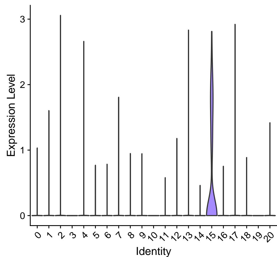
CD8B
